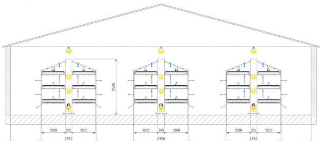
Three tier aviary system
