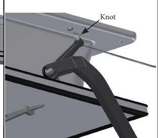
Step 9: (Shut-off)
